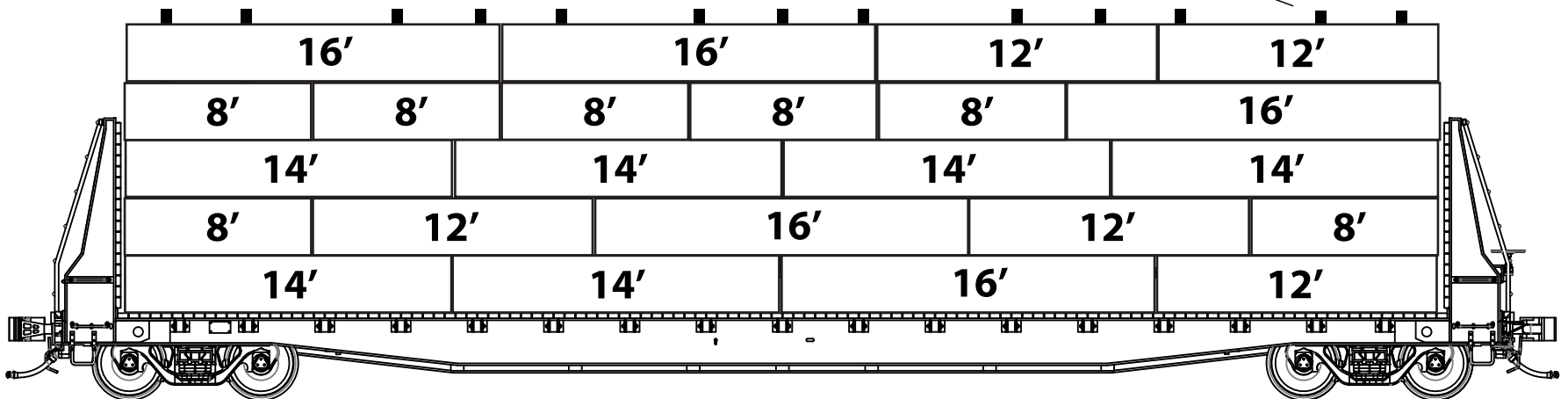
Sleepers are not shown for clarity. Stacks represents the overall envelope clearance. © Wheels of Time
